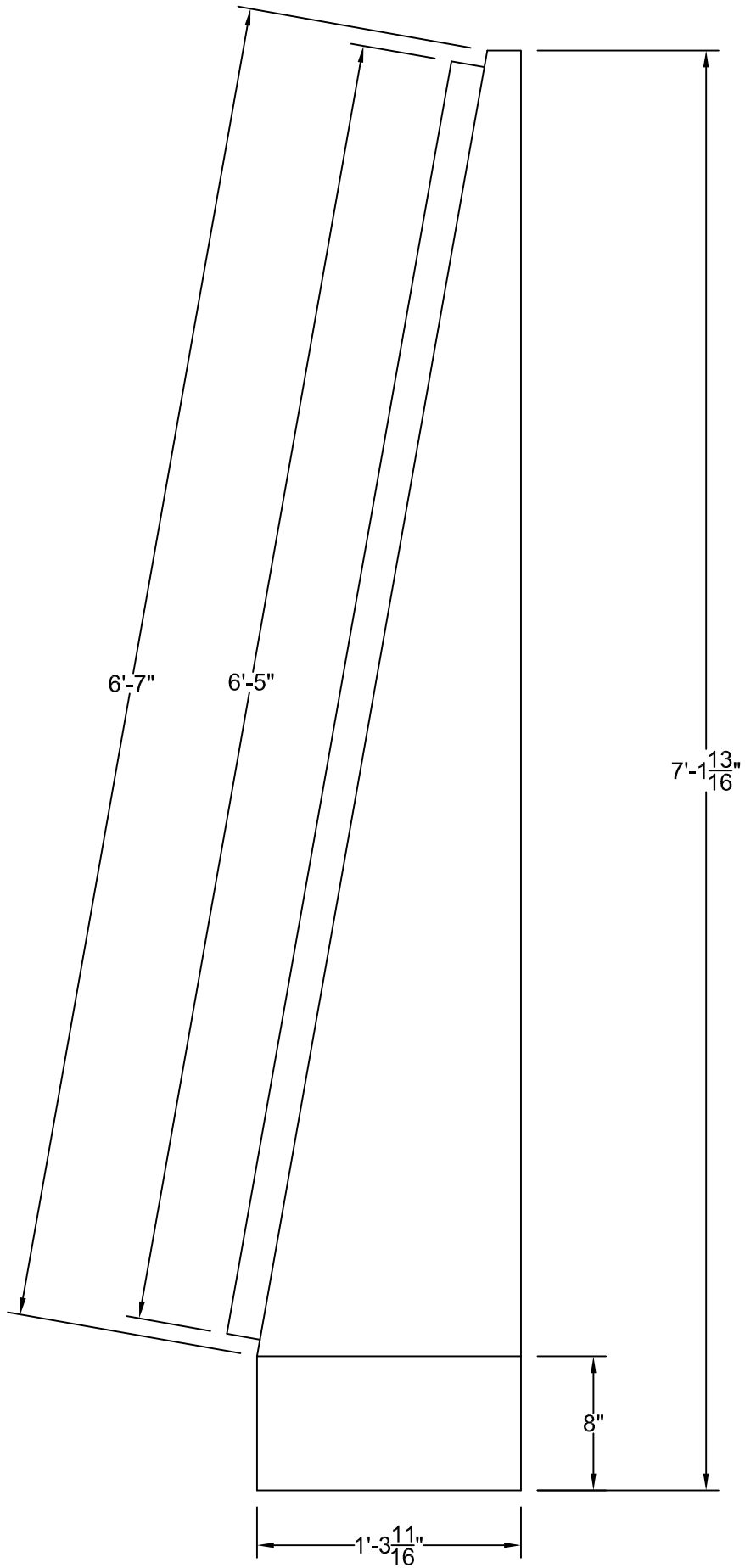
PEDESTAL SIDE VIEW REV G, 220317
